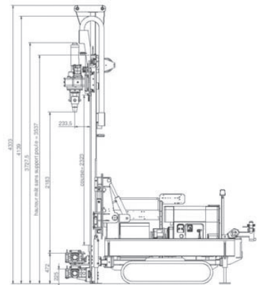
Dimensions on working position
