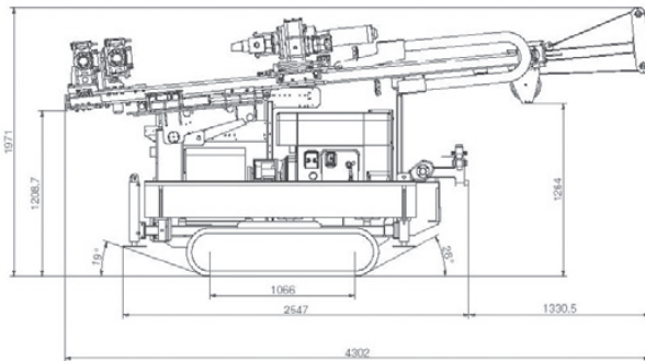
Dimensions on displacement position
